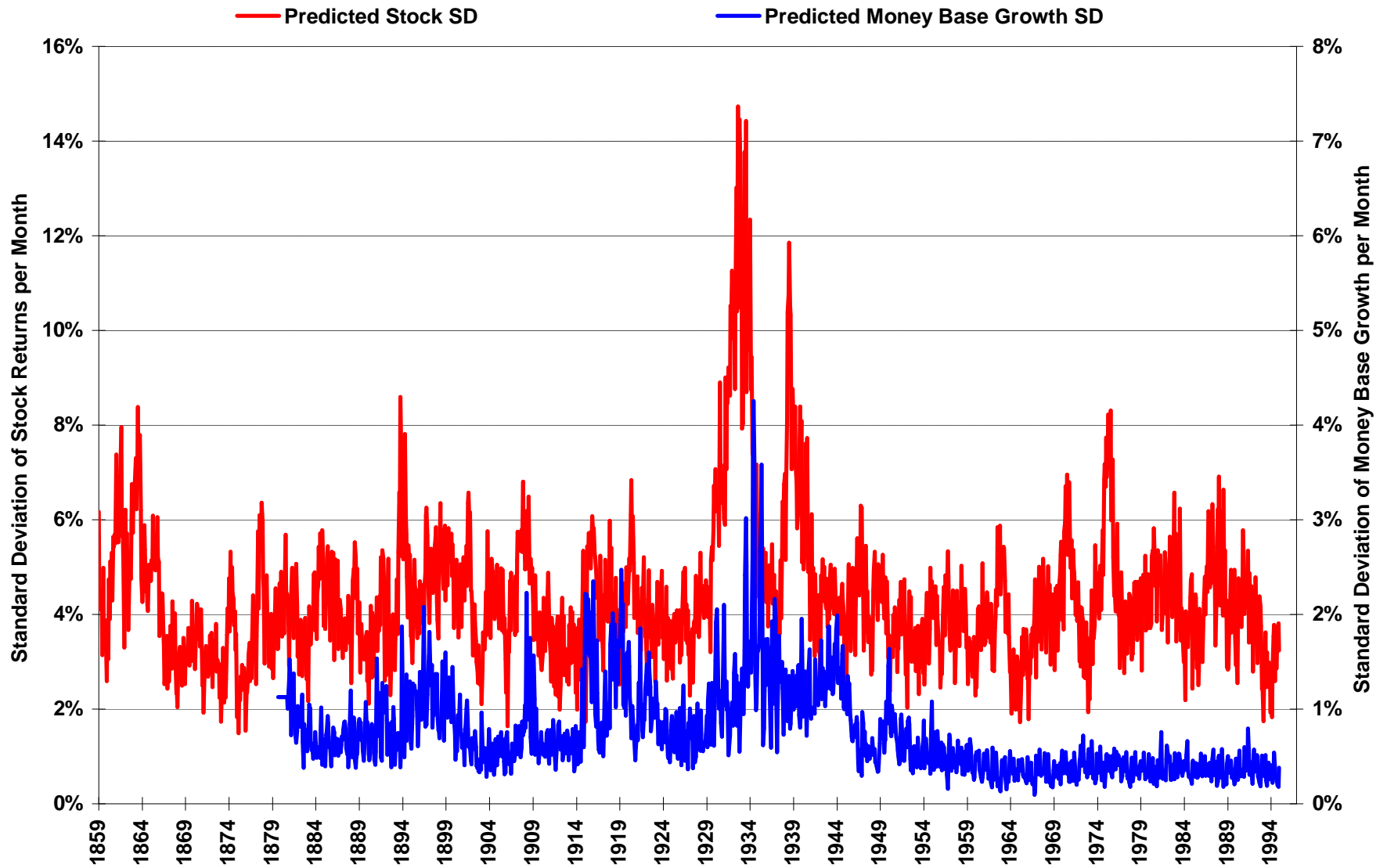
Fig. 5 -- Predicted Stock Return and Money Base Growth Volatility
